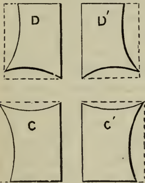
FIG. 143.—Method of shaping the Corner Blocks.
